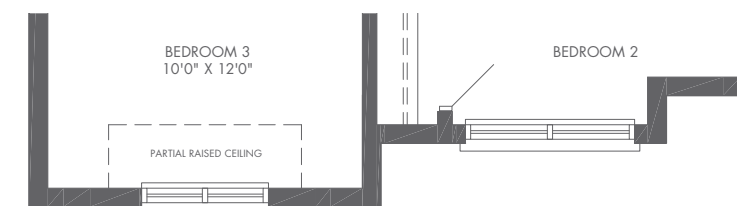
2ND FLOOR ELEV. B PARTIAL
